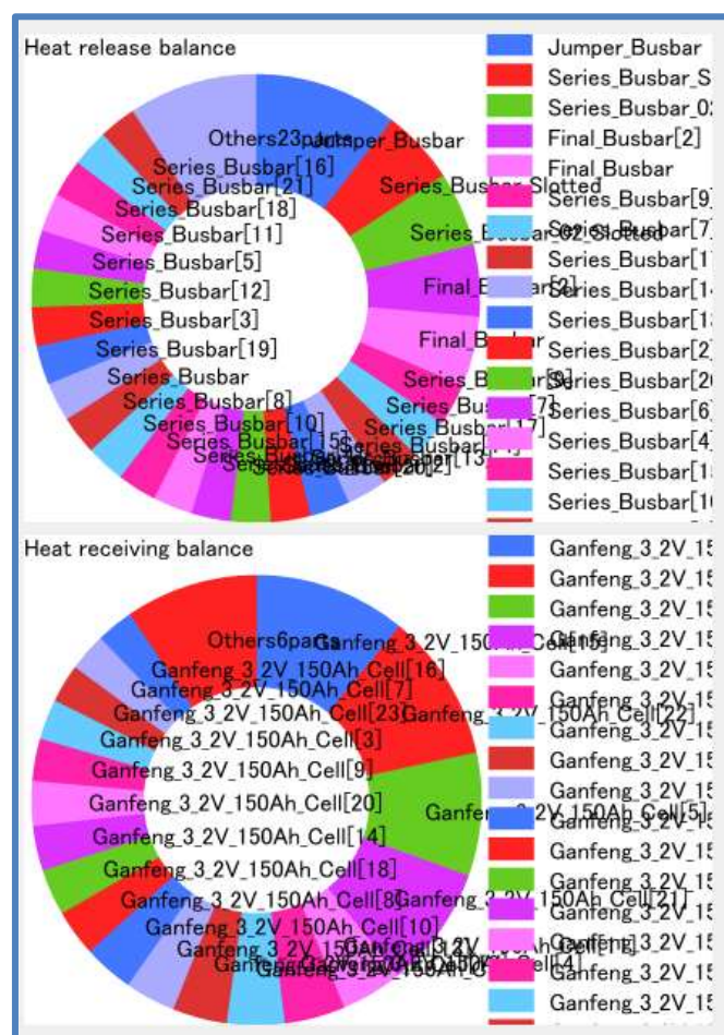
Figure 12: Heat balance information of each part during discharging cycle
