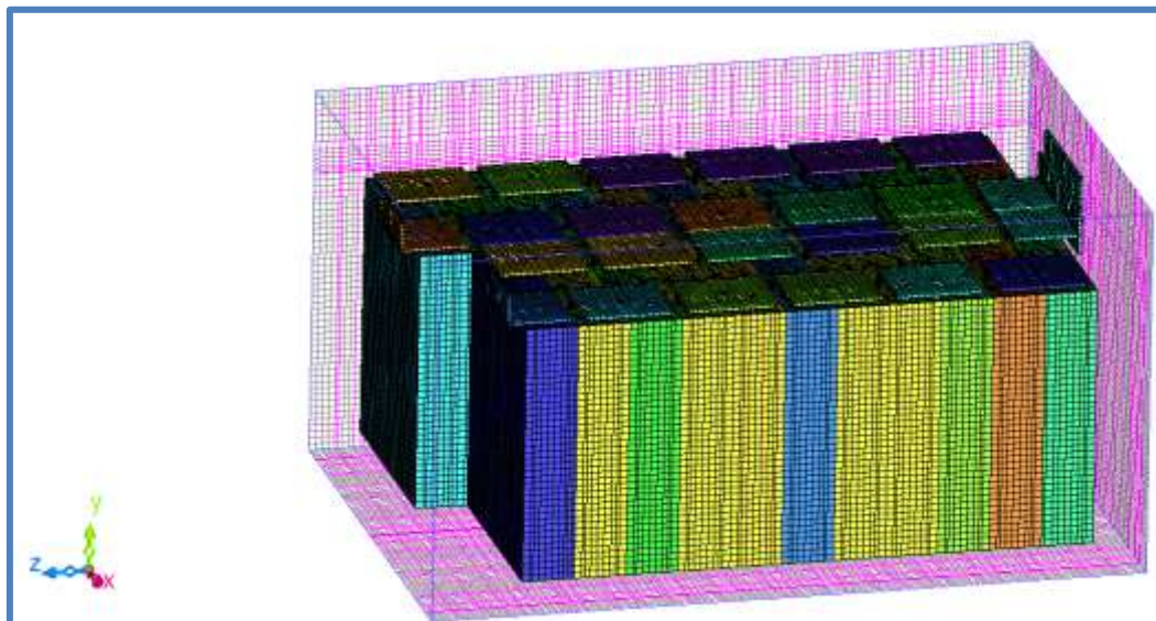
Figure 2: Mesh Model Isometric view
