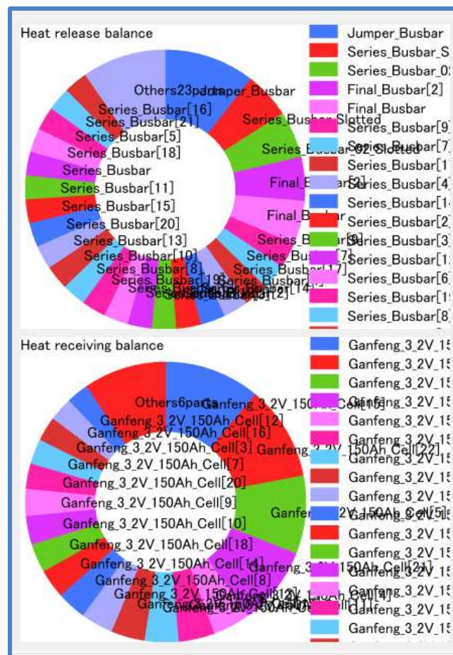
Figure 10: Heat balance information of each part during Charging cycle
