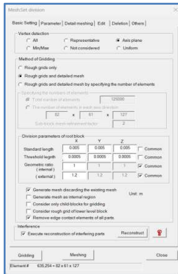
Figure 5: Mesh Conditions
