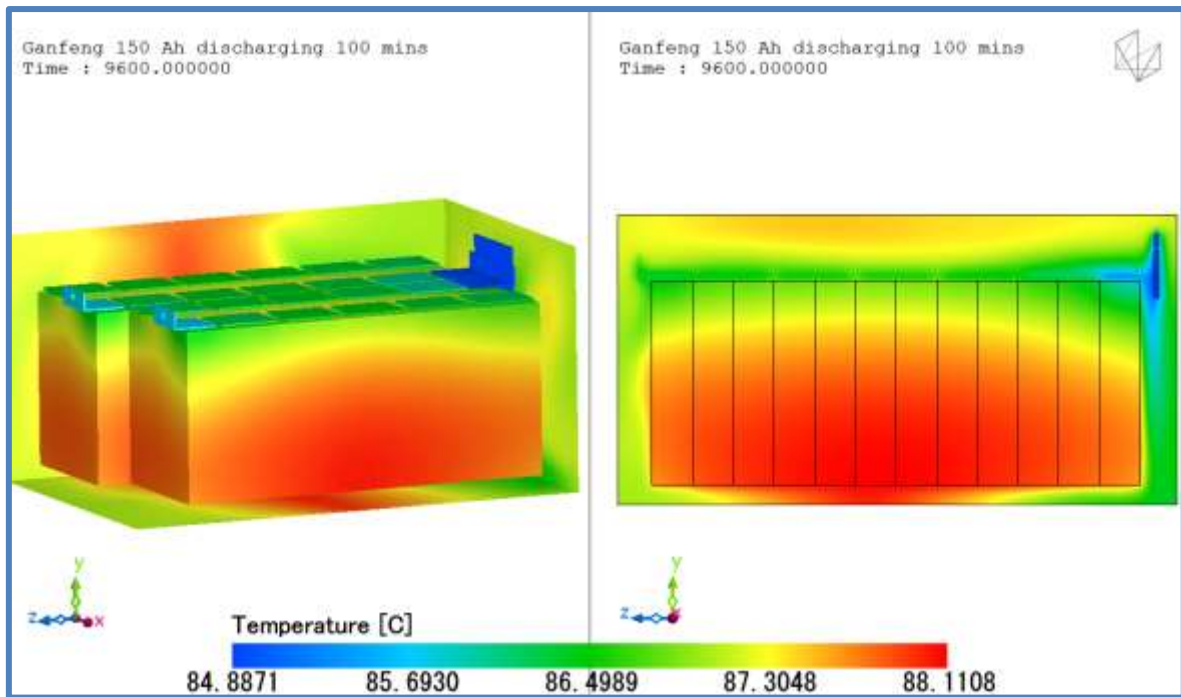
Figure 8: discharging Temperature Contour of different view
