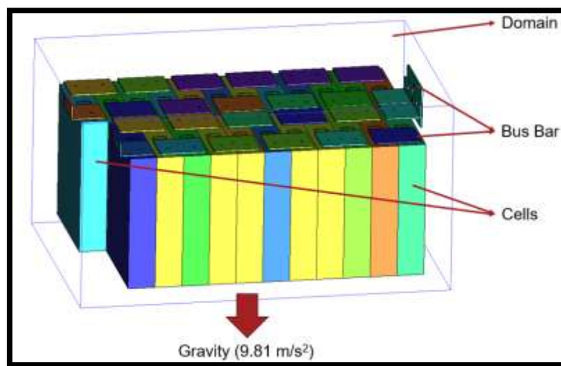
Figure 1: Battery Model
