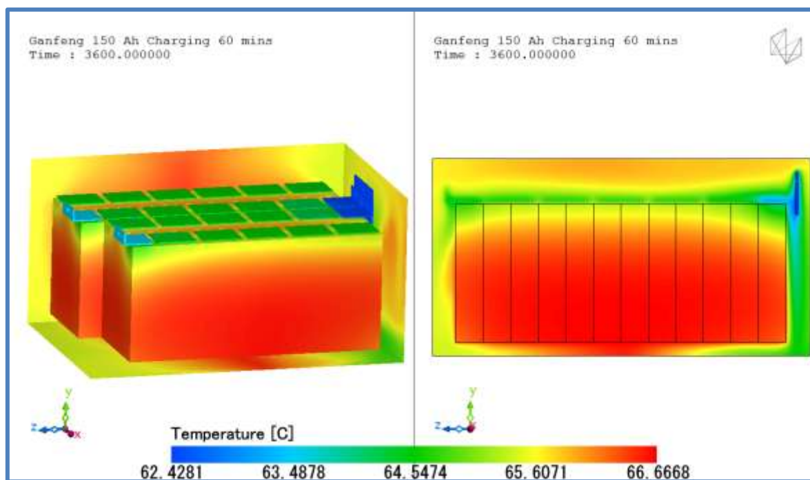
Figure 7: Charging Temperature Contour of different view
